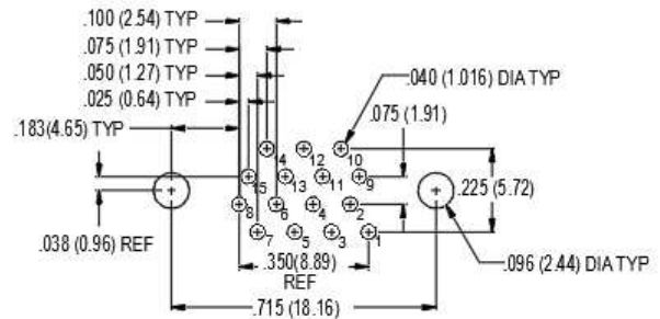
15 PIN M83513/28-B
