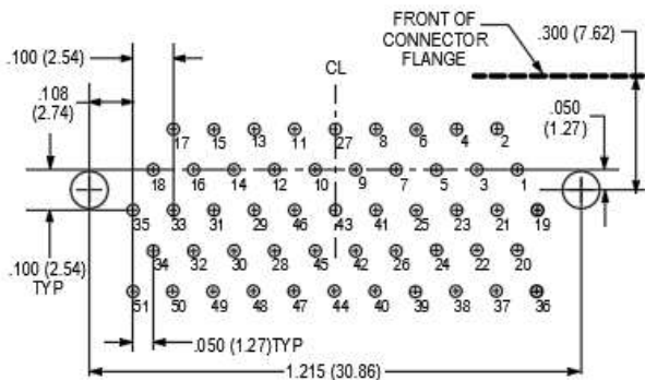
51 SOCKET M83513/14-G
