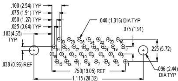
31 PIN M83513/28-E
