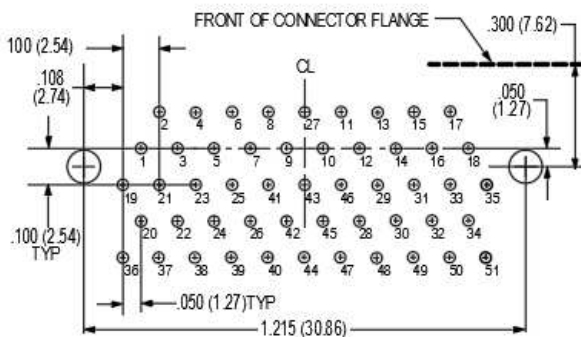
51 PIN M83513/11-G
