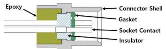
[Socket Connector]
