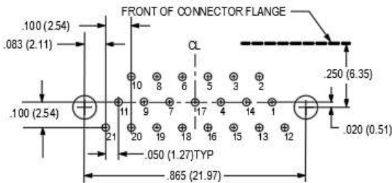
21 SOCKET M83513/13-C
