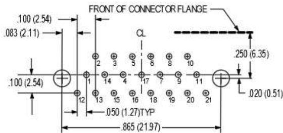
21 PIN M83513/10-C
