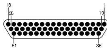
G - 51 Contacts
