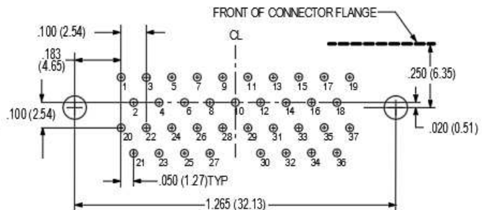
37 PIN M83513/10-F
