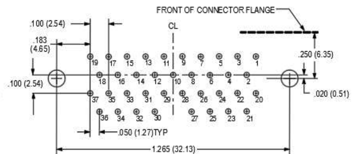
37 SOCKET M83513/13-F
