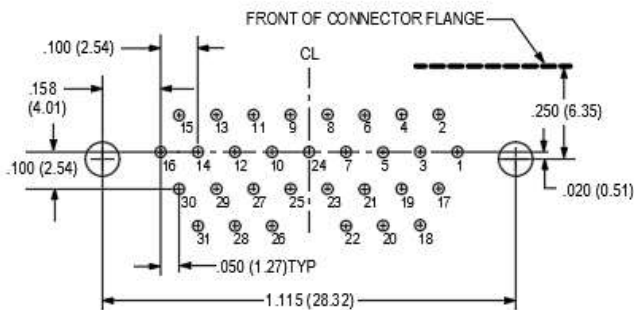
31 SOCKET M83513/13-E
