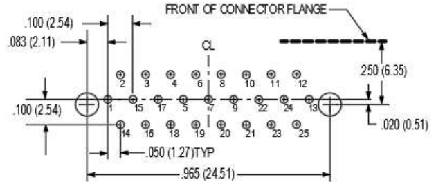
25 PIN M83513/10-D
