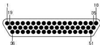
G - 51 Contacts
