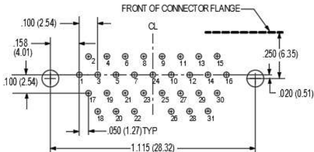
31 PIN M83513/10-E
