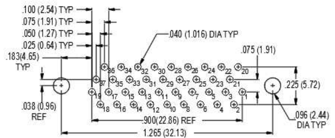
37 PIN M83513/28-F
