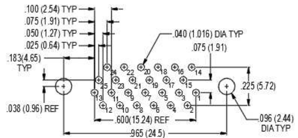
25 PIN M83513/28-D
