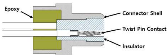
[Pin Connector]
