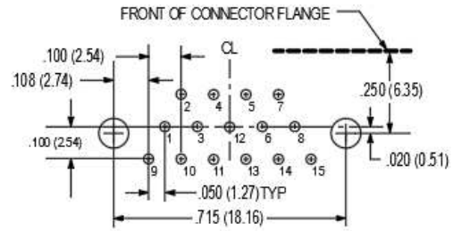
15 PIN M83513/10-B
