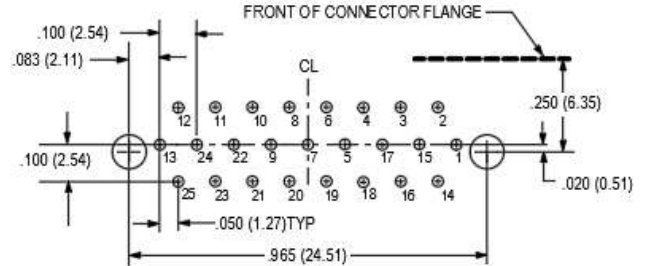
25 SOCKET M83513/13-D
